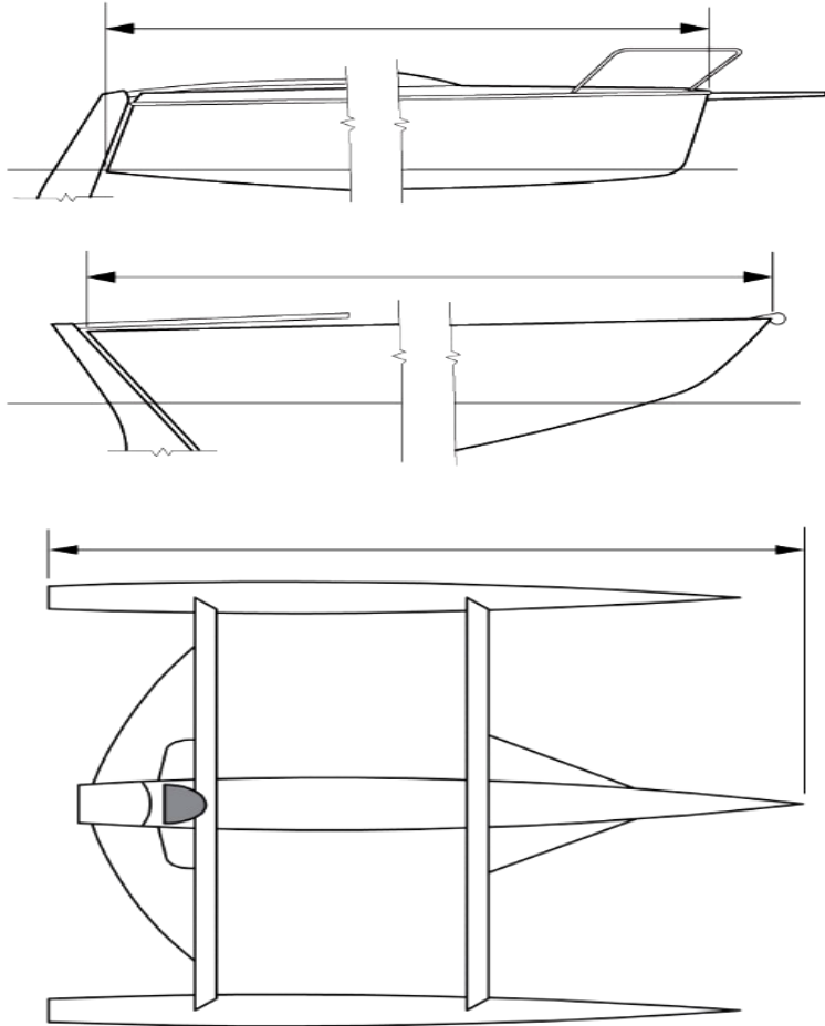
Hull Length
